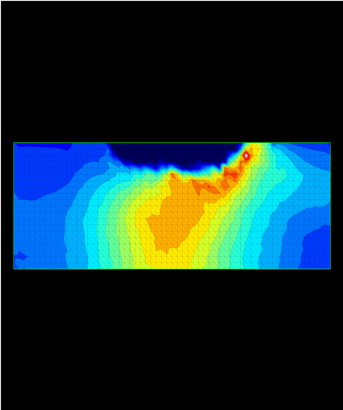
Figure 8.7: MESFET Fast Monte Carlo Energy Profile computed by Archimedes .
