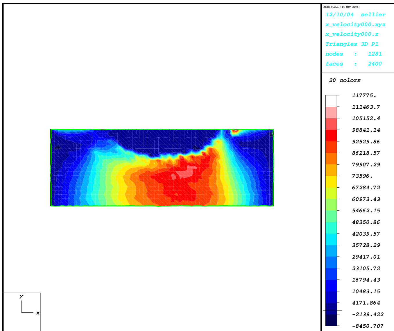
Figure 8.2: MESFET x-component velocity computed by Archimedes.
