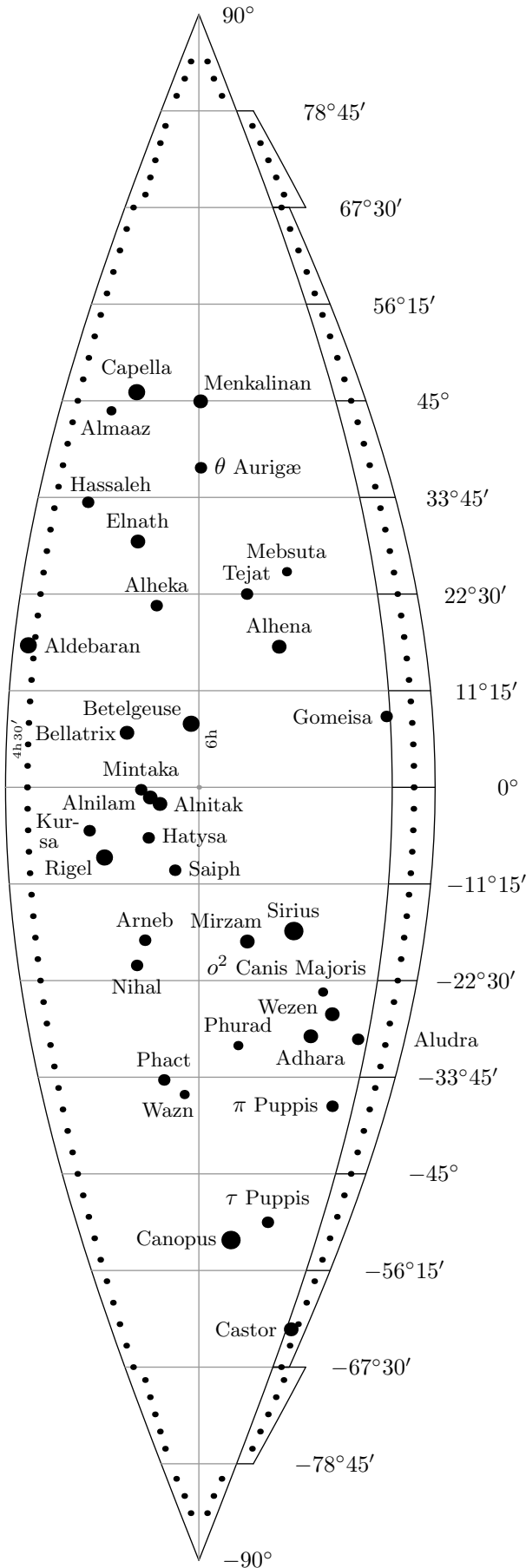
3 RA 4h 30' 6h 7h 30' 67.5° 90.0° 112.5°
