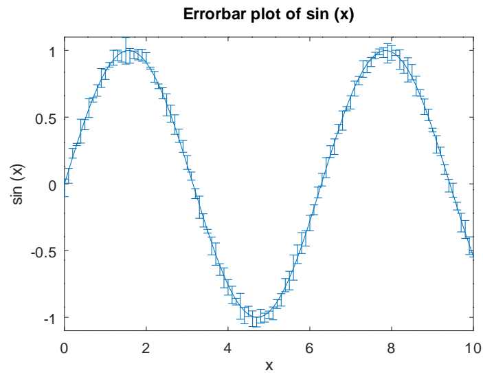
Figure 15.3: Errorbar plot.
