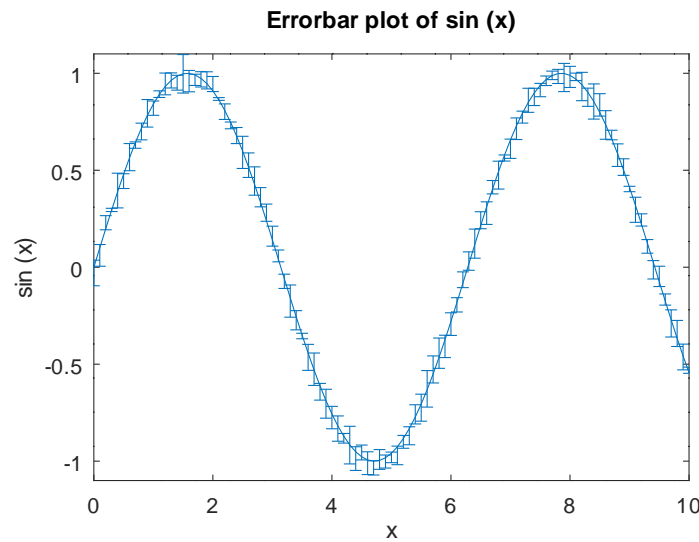
Figure 15.3: Errorbar plot.
