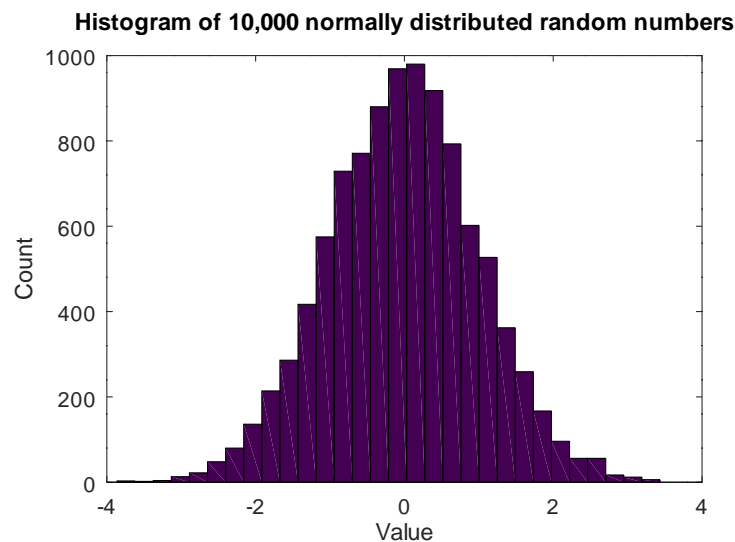
Figure 15.2: Histogram.
