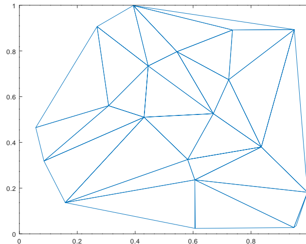
Figure 30.2: Delaunay triangulation of a random set of points
