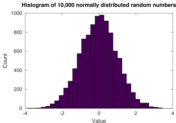
Figure 15.2: Histogram.
