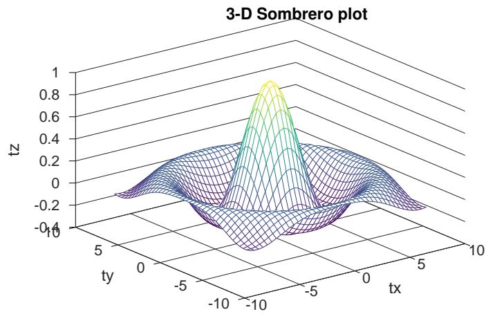
Figure 15.5: Mesh plot.
